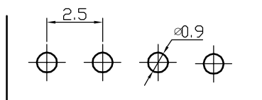
PCB Layout
