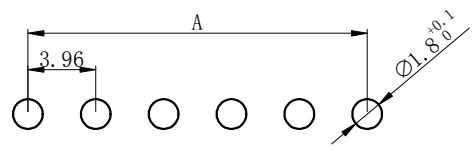
P. C. B Board Layout (t=1.6mm)
